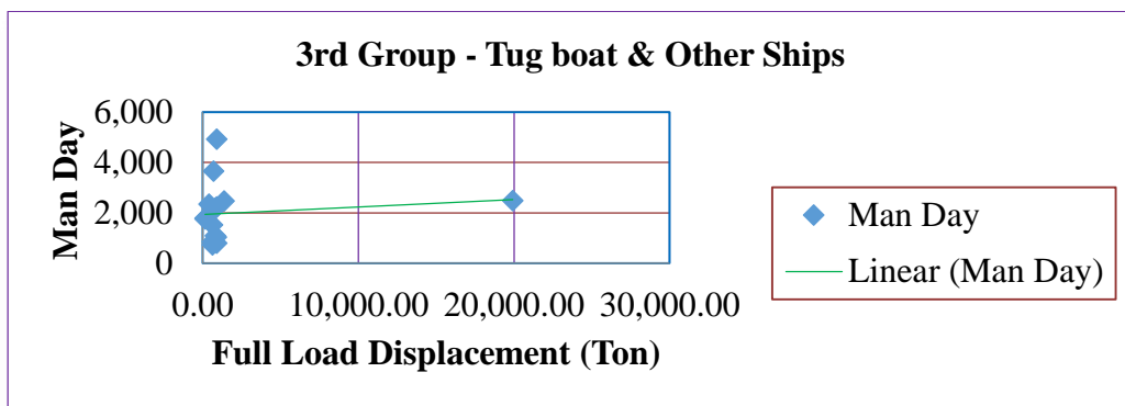
Figure – 52: Man Day vs Full Load Displacement (Ton)
