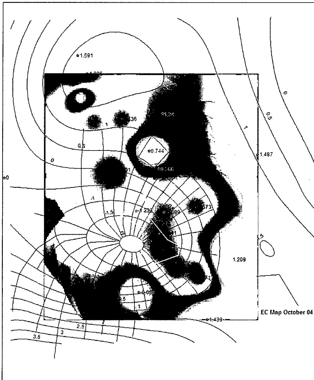
Figure 5-34 Iso-piezometric Flow Lines for October, 2004
