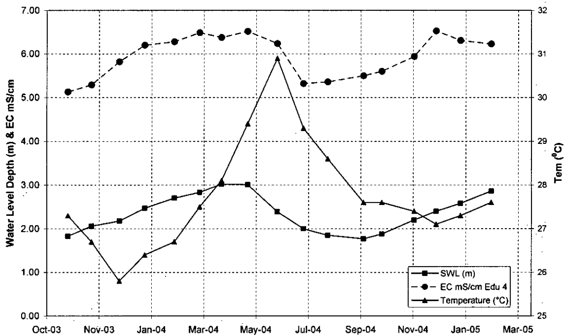
Figure 5-10 Upper Shallow Aquifer Water Level Depth (well top), EC and Temp. at Edu_04
