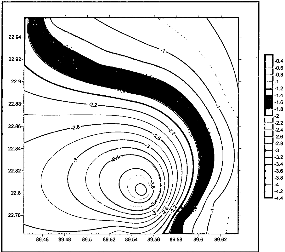
Figure 5-33 Iso-Piezometric thematic Map of SWL for April, 2009 for the Deep Aquifer
