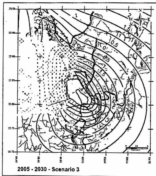
Figure 5-46 BRGM-ANTEA-ARMCO Modelling Scenario 1, 2 and 3
